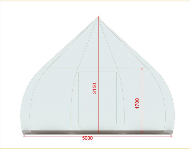
Water drop starry sky tent dimensions
