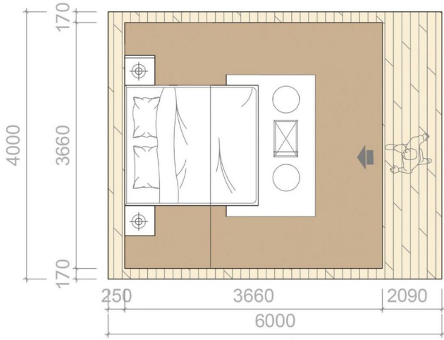
K -200 Tent Drawing
