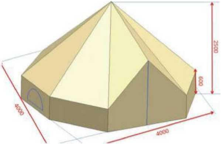
BELL-400 Tent dimensions
