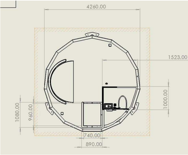
Star Capsule inner drawing
