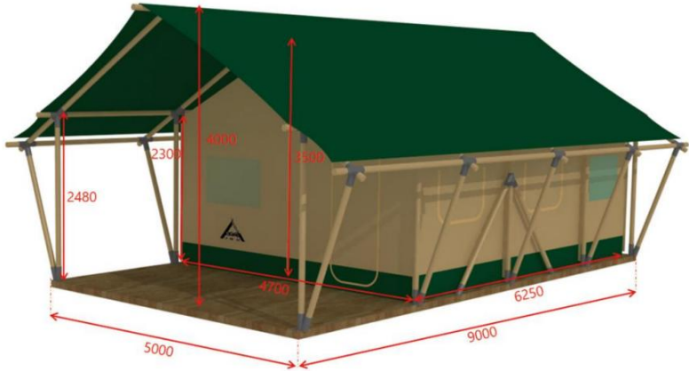
M-8 Tent Dimensions
