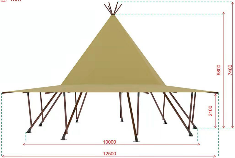
Tent deployment size
