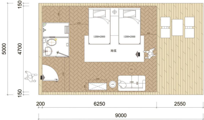
M-8 Tent Indoor Drawing
