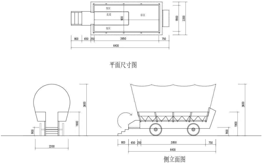
carriage tent Tent Indoor Drawing
