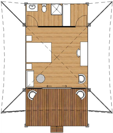
M13 Tent Indoor Drawing
