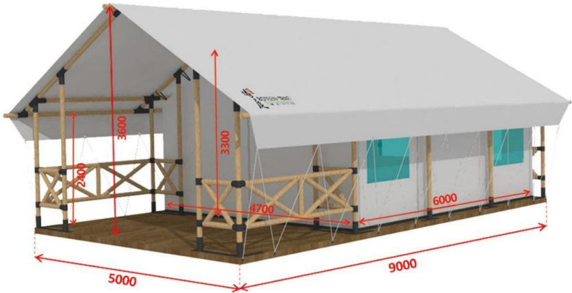
M-8 Duplex Tent Dimensions
