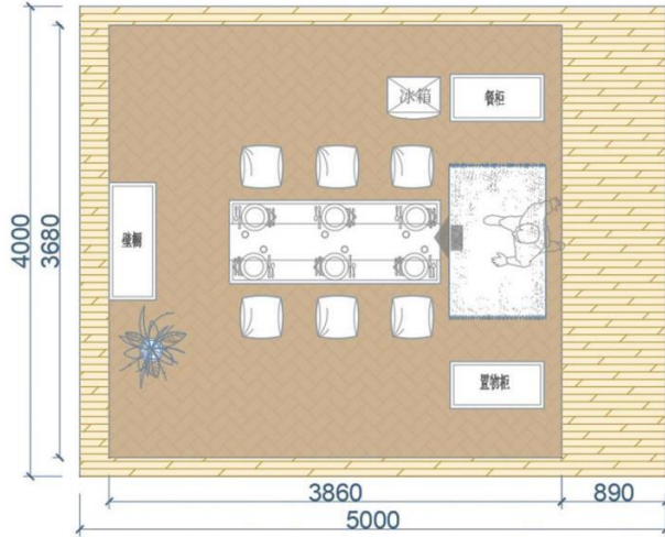
Small A Tent Drawing
