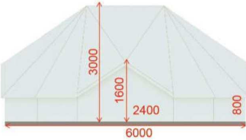
BELL-460 Tent dimensions
